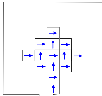
Parallel/chessboard-style installation of modules
